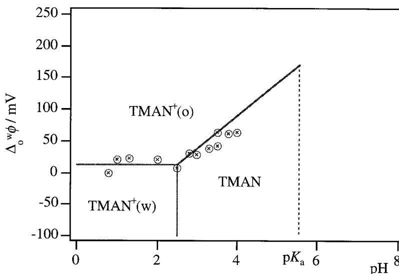
Fig. 3. Ionic partition diagram of tetramethylaniline ( \text{BH}^+ ) at the water–nitrophenyloctyl ether interface obtained with the microfilter plate system. The dotted line at the right side shows the aqueous \text{p}K_a value.
